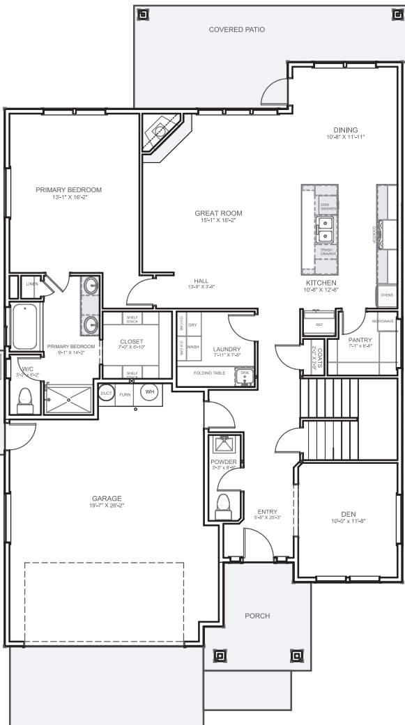
MAIN FLOORPLAN
